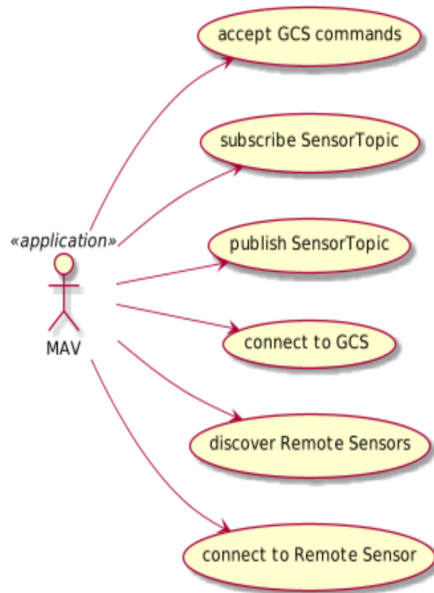
Figure 5: Use-case diagram of the MAV
