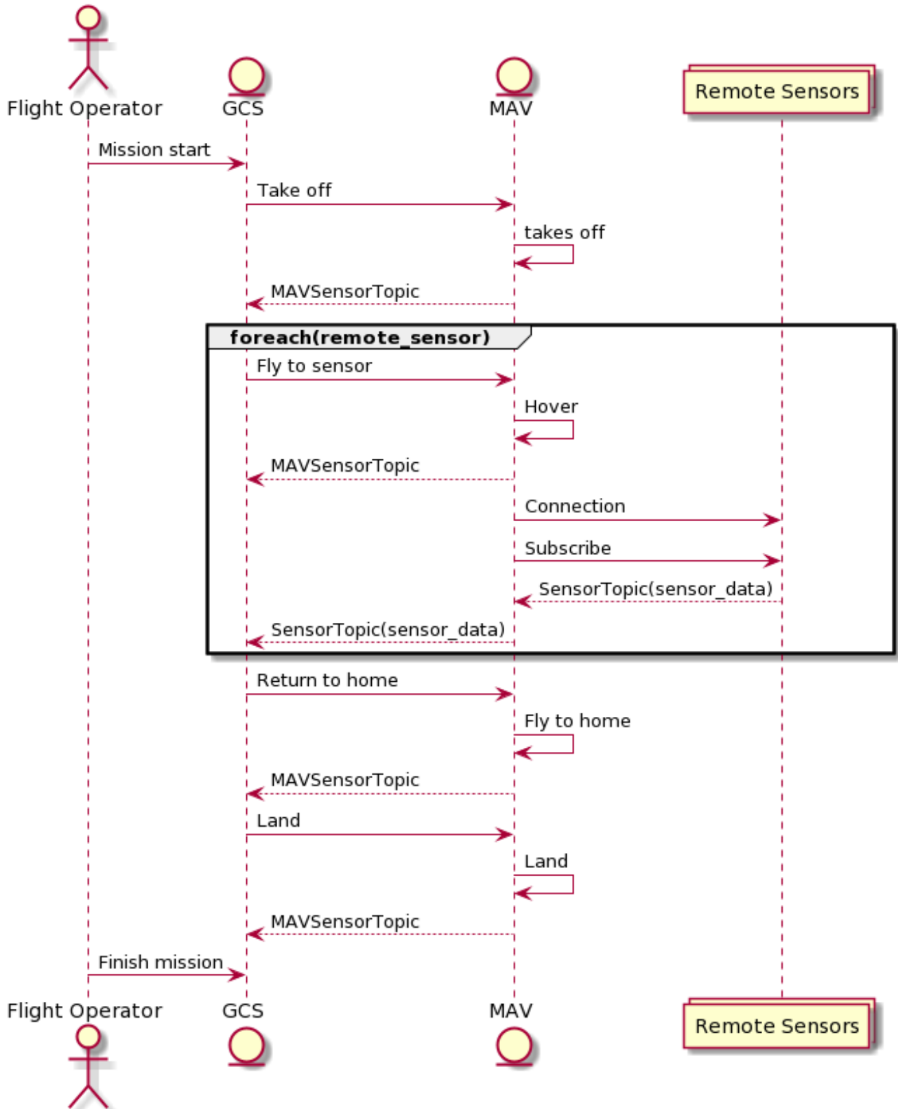
Figure 1: Use-case as sequence diagram
