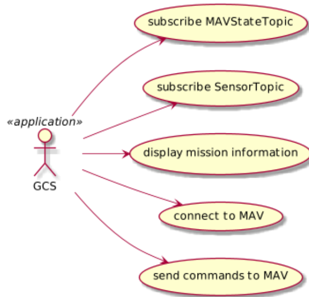
Figure 3: Use-case diagram of the GCS
